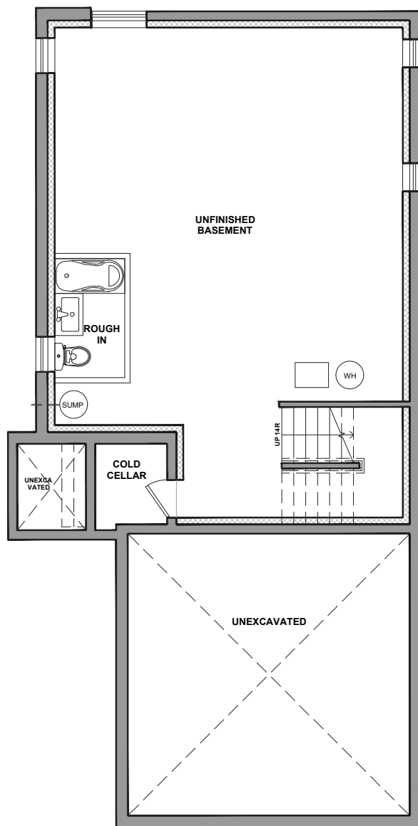
BASEMENT PLAN
