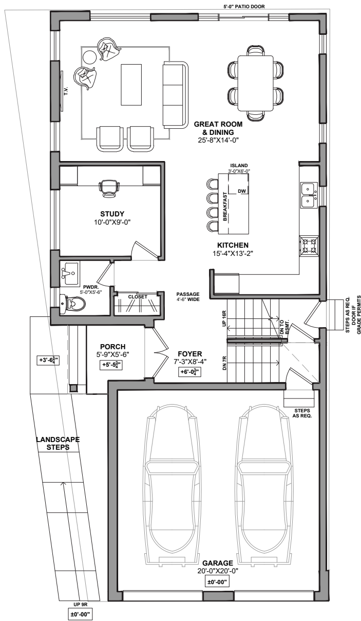
FIRST FLOOR : 937 SQ.FT.
